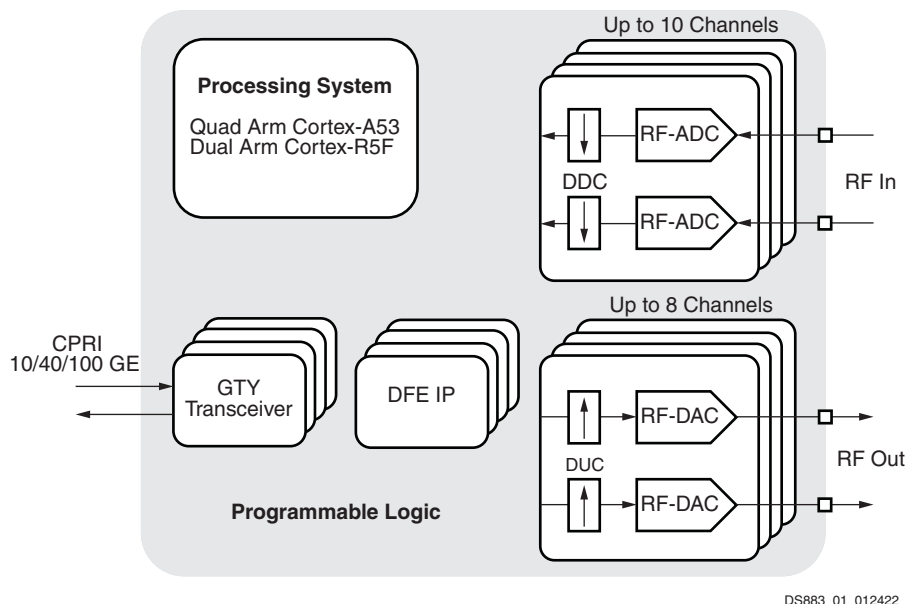
Figure 1: Zynq UltraScale+ RFSoc DFE
