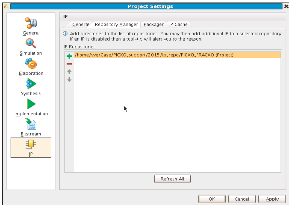
Figure 18: Project Settings
