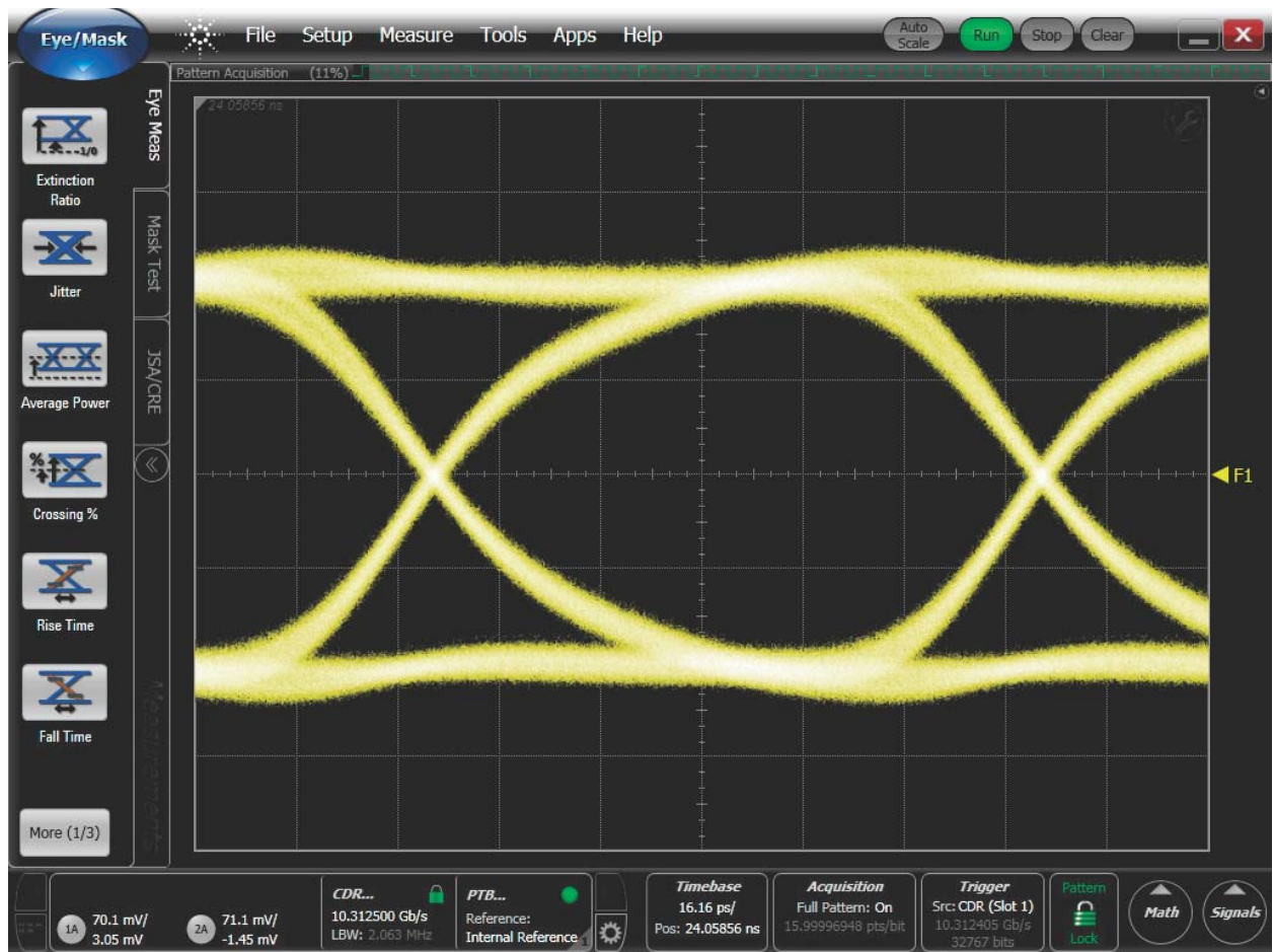
Figure 10: 10.3125 Gb/s Output
