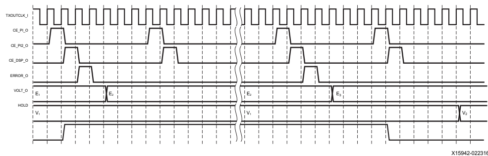
Figure 16: HOLD Input Operation
