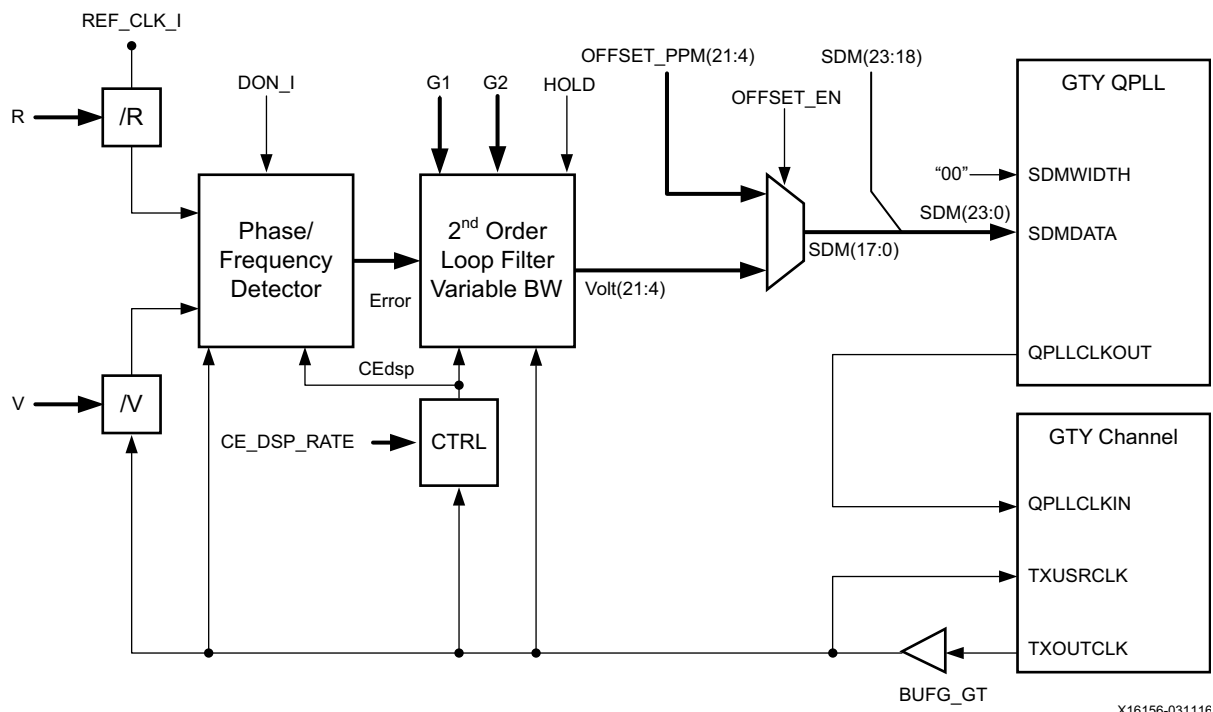
Figure 12: DPLL for GTY Transceiver in UltraScale Devices
