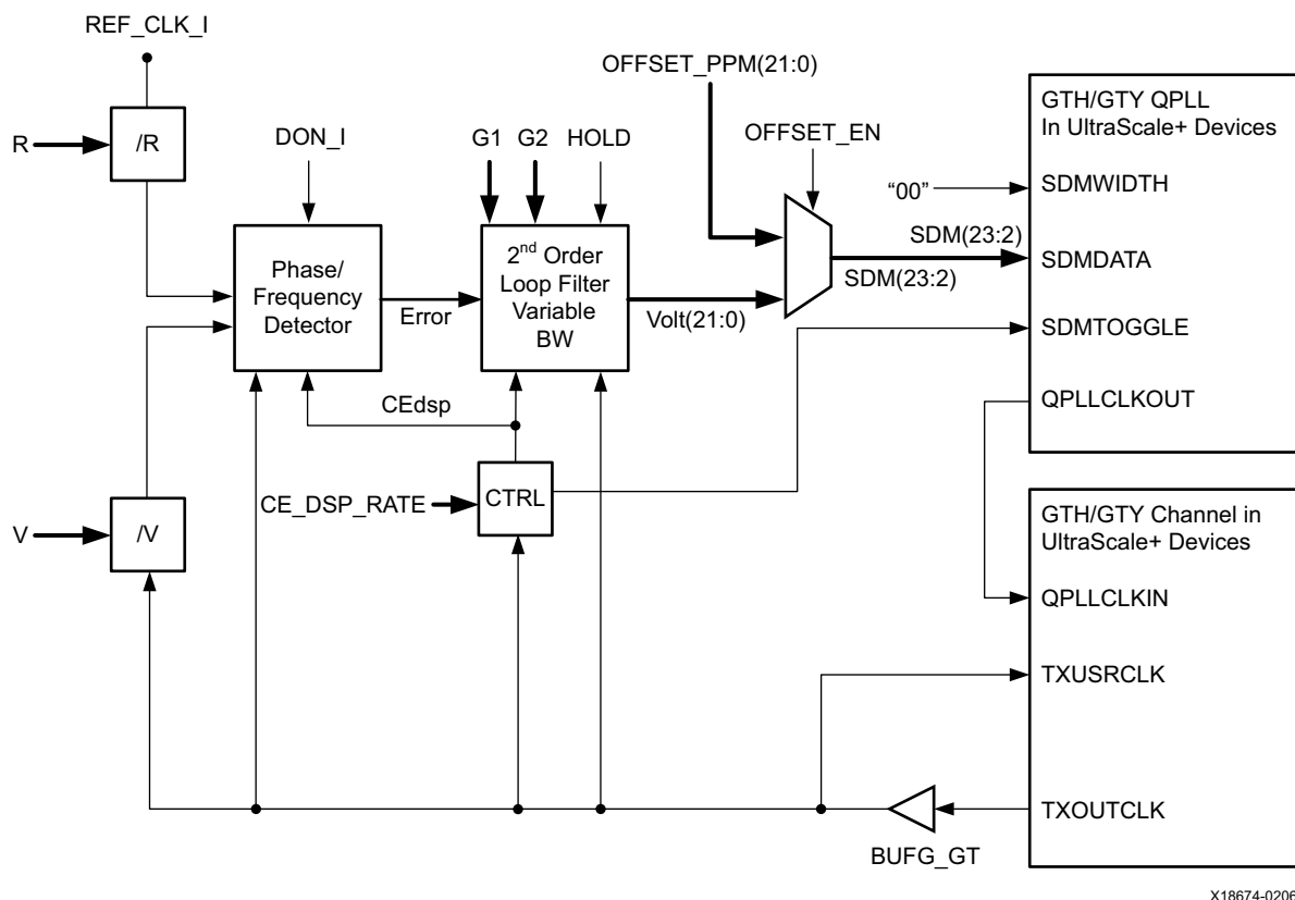
Figure 13: DPLL for GTH and GTY Transceivers in UltraScale+ Devices
