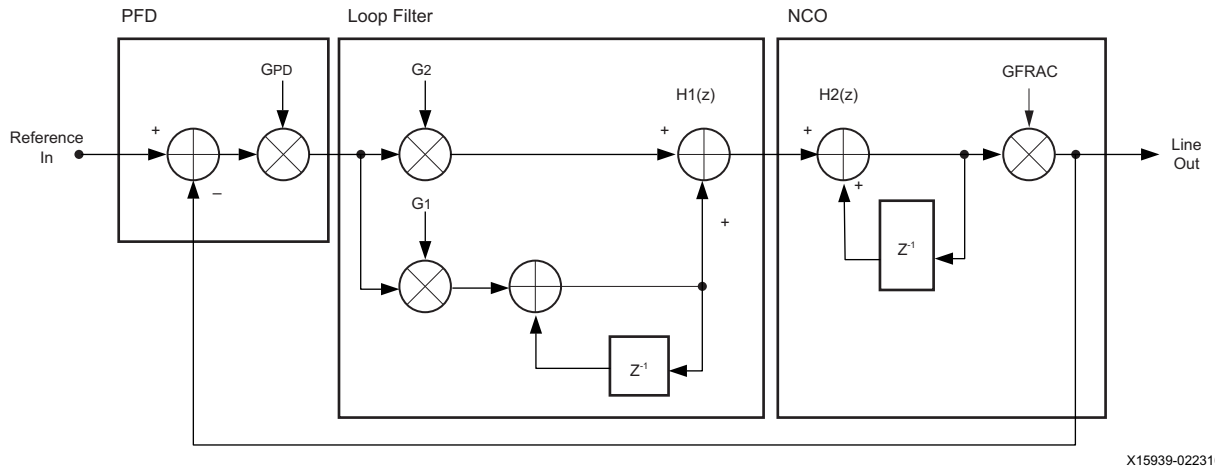
Figure 3: FRACXO DPLL Digital Equivalent
