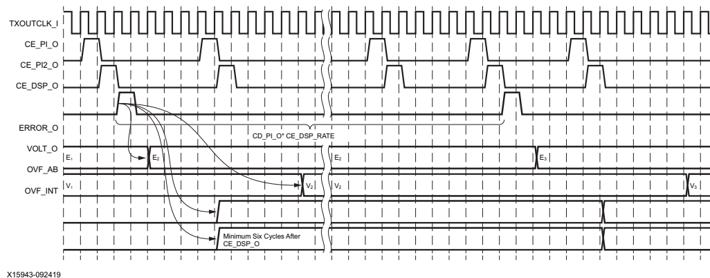
Figure 17: Direct Offset Control
