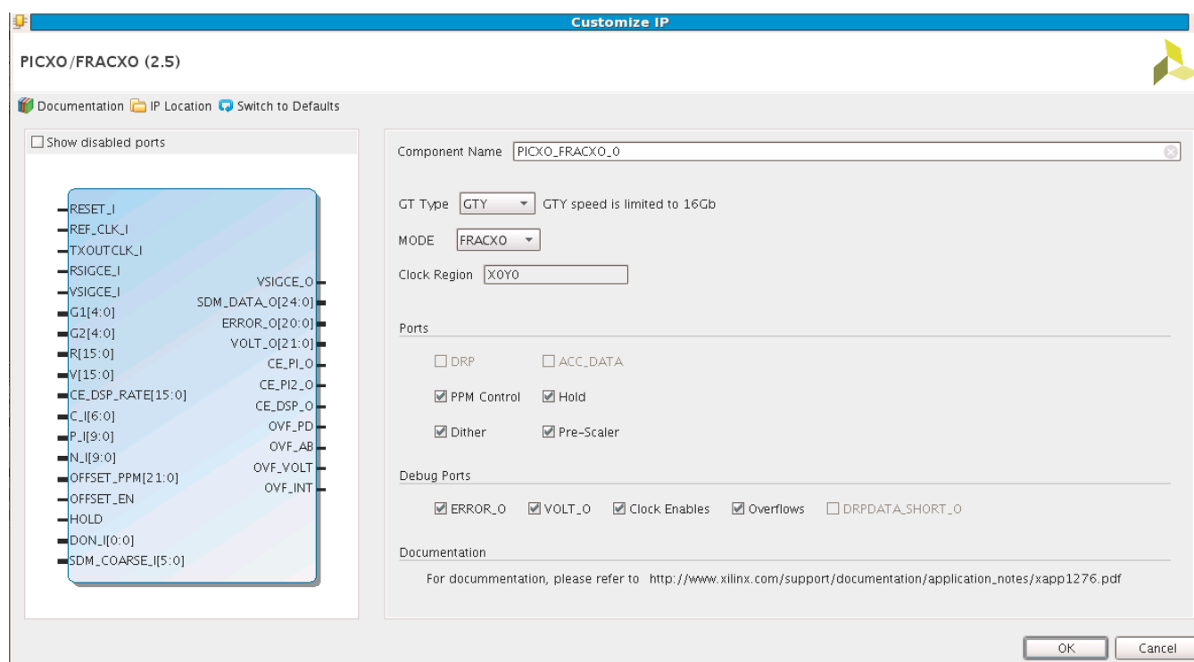
Figure 20: Customize IP
