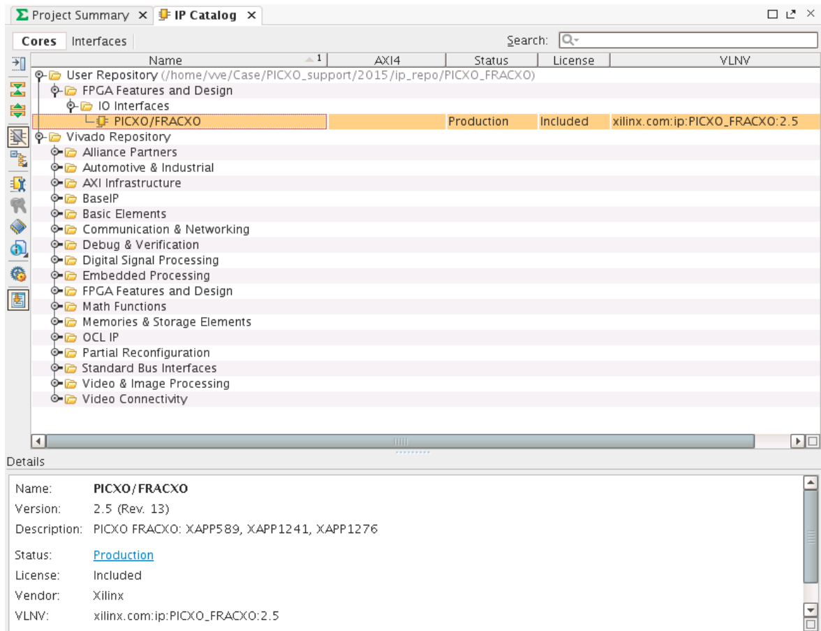
Figure 19: IP Catalog
