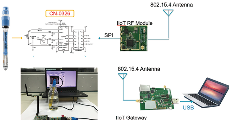
Fig.1 pH sensor+CN0326+IIoT Module
